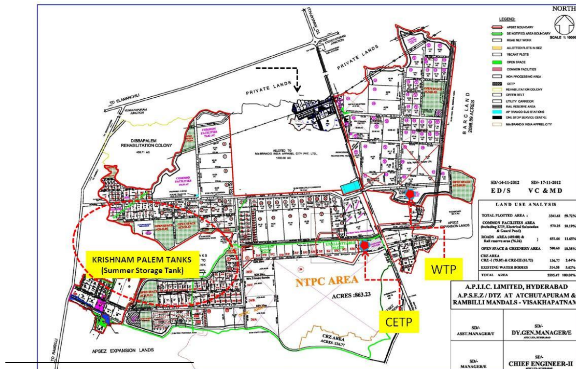
Figure 1: Schematic Layout of Atchutapuram SEZ depicting CETP Location
